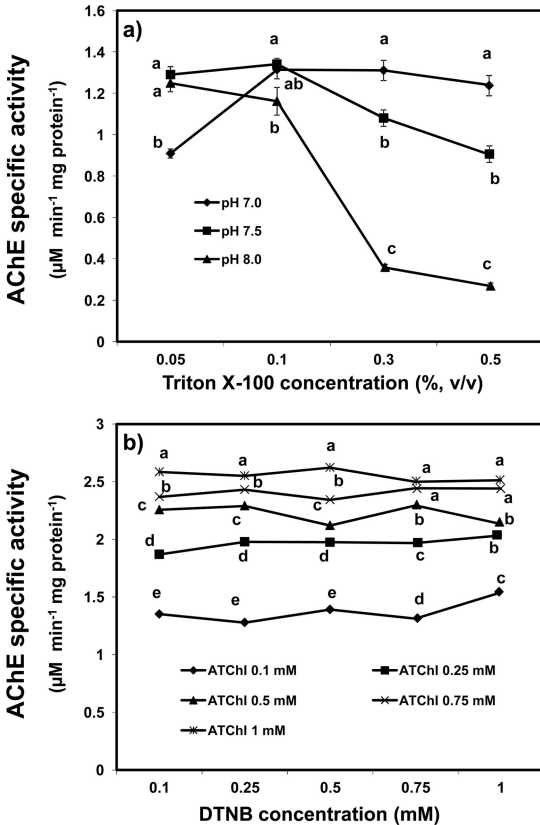
Fig. 1. Effect of (a) Triton X-100 concentration and phosphate buffer pH, and (b) DTNB and ATChI concentrations on specific activity of AChE. Each symbol represents mean ± SEM ( n = 4-13 ). Symbols labeled with a different letter within a given concentration of Triton X-100 or DTNB are significantly different from one another according to LSD ( P < 0.05 ).
