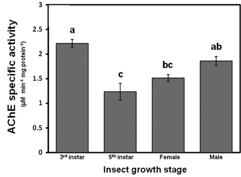
Fig. 2. Effect of D. citri growth stage on specific activity of AChE. Each bar represents mean ± SEM ( n = 7-15 ). Bars labeled with different letters are significantly different from one another according to LSD ( P < 0.05 ).
