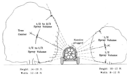
Figure 1. Recommended nozzle arrangement and spray volume distribution.
